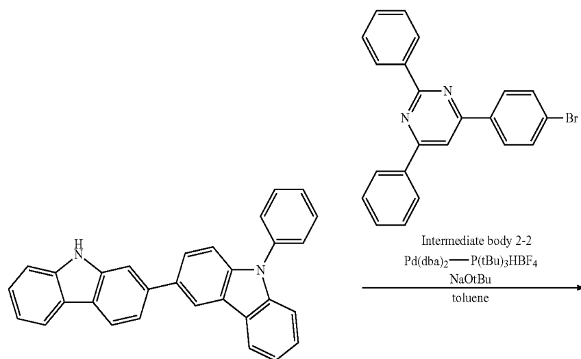
Intermediate body 1-4
