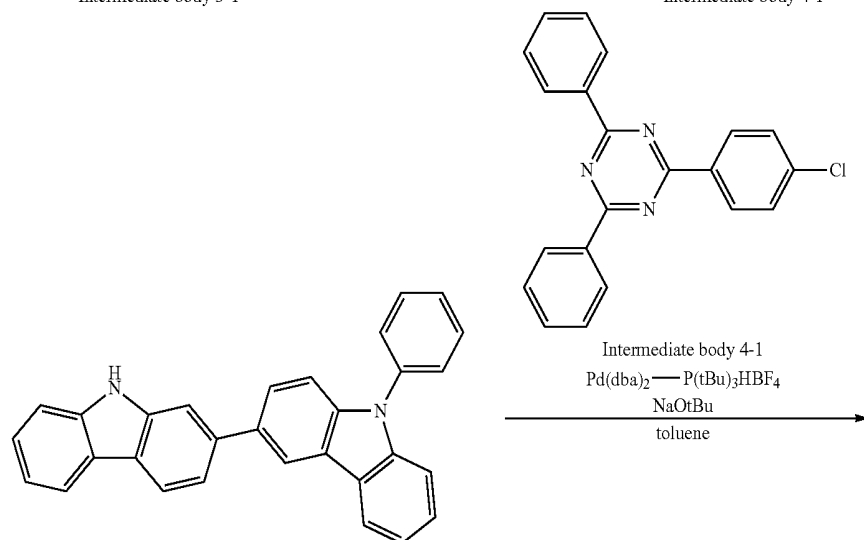
Intermediate body 1-4
