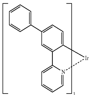
Ir(Ph-ppy) 3 (facial body)
