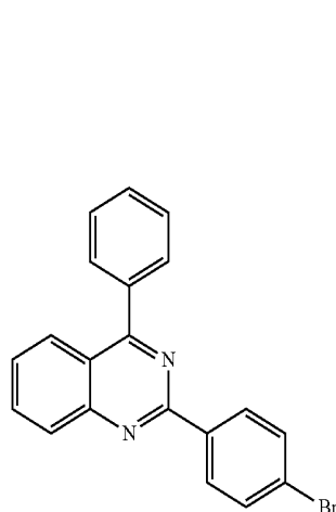
Intermediate body 7-1
