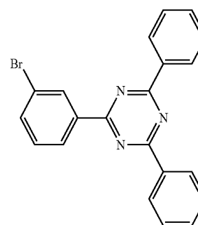
Intermediate body 5-2
